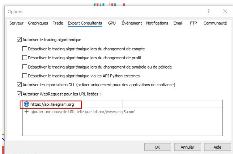
Figure 6 — Expert Advisors tab: enable Allow WebRequest and add https://api.telegram.org .
